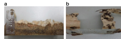
○ Examples of the range of termite attack and damage to non-treated Radiata pine sapwood control test specimens after exposure to C. acinaciformis in a Hazard Class H3 field trial for 38 weeks: a) 86.5% mass loss, and b) 99.3% mass loss. (Mean mass loss for seven test specimens = 95.5%).
