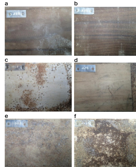
○ Example of termite attack to treated test specimens after exposure to C. acinaciformis in a Hazard Class H3 field trial for 38 weeks: a) Abodo Vulcan Radiata 230°C TPX uncoated, b) Abodo Vulcan Radiata 230°C TPX stained, c) Abodo Vulcan Radiata 230°C TPX painted, d) Radiata pine, uncoated, e) Radiata pine TPX, uncoated, LOSP, and f) Radiata pine, painted, LOSP.
