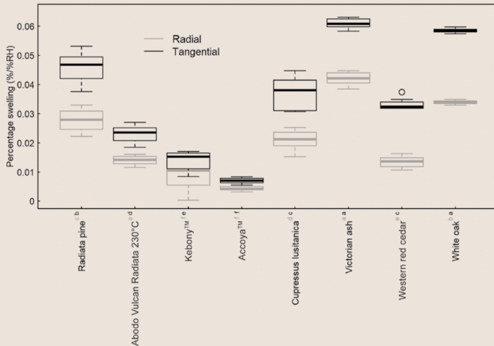
FIGURE 2. Percentage swelling for every 1% change in relative humidity for each wood type in the tangential and radial directions (shown as black and grey boxes respectively). Superscript letters indicate grouping that are not significantly different (95% confidence level).
