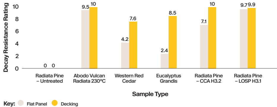
Graph 4: Flat Panel and Decking – Condition of Samples After 7+ Years
