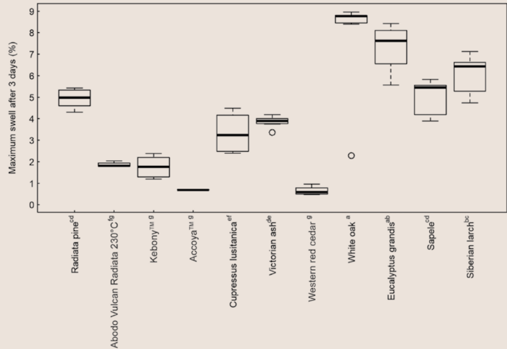
FIGURE 1. Maximum swelling following 3 days water soaking in the Swellometer test. Superscript letters indicate grouping that are not significantly different (95% confidence level).
